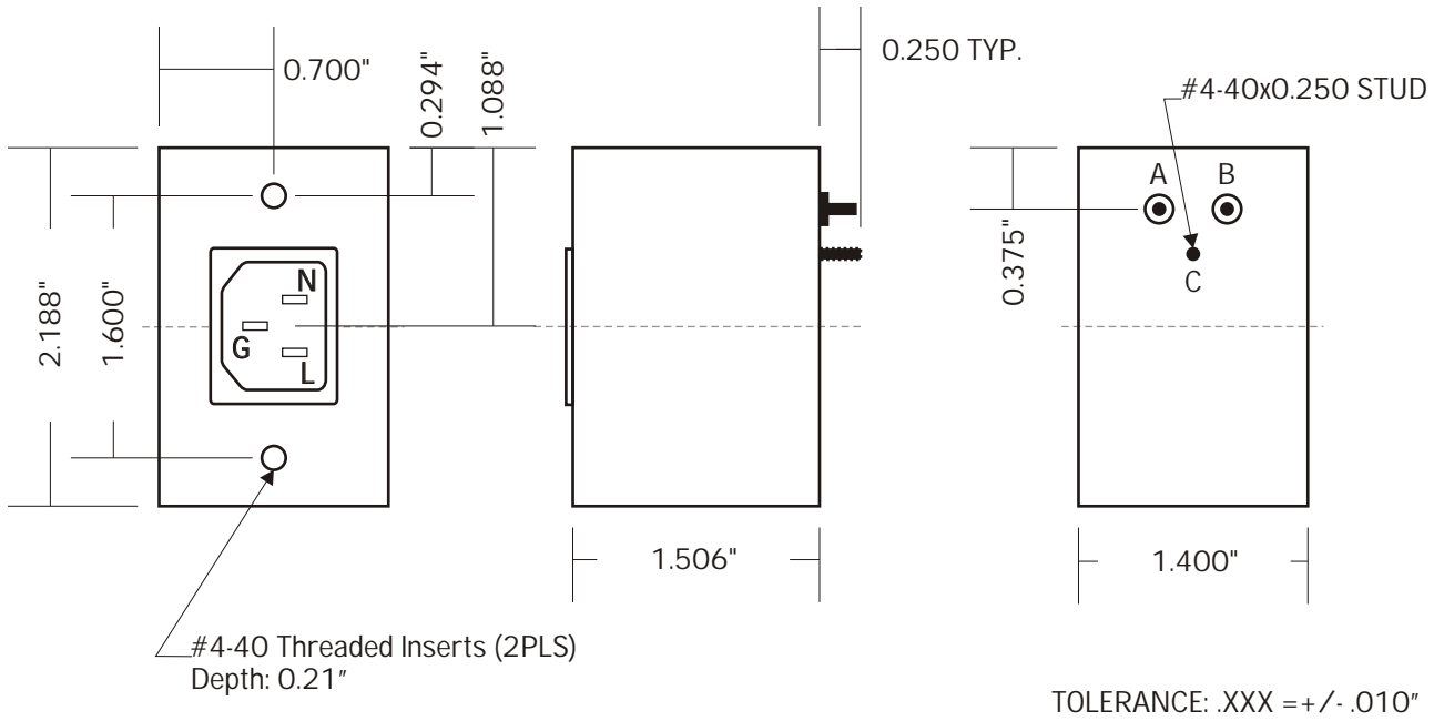
OUTLINE DRAWING
