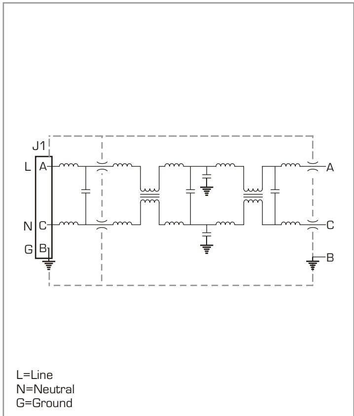
FUNCTIONAL DIAGRAM
