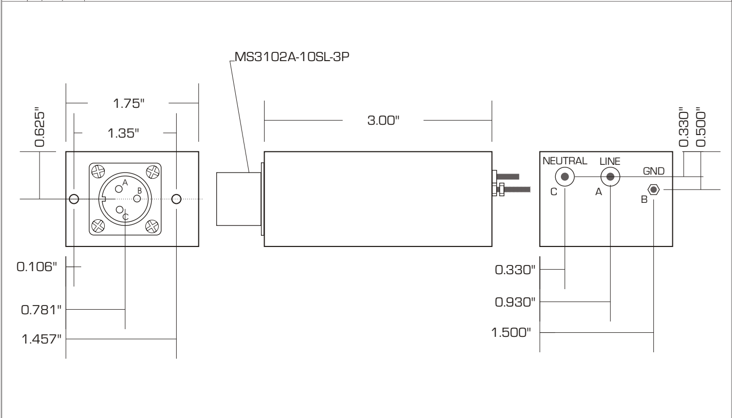
OUTLINE DRAWING
