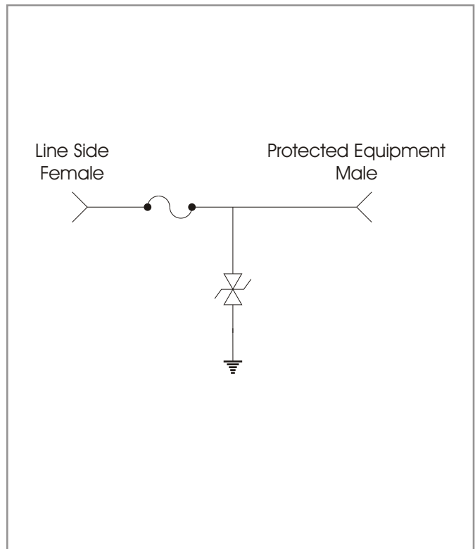
FUNCTIONAL DIAGRAM
