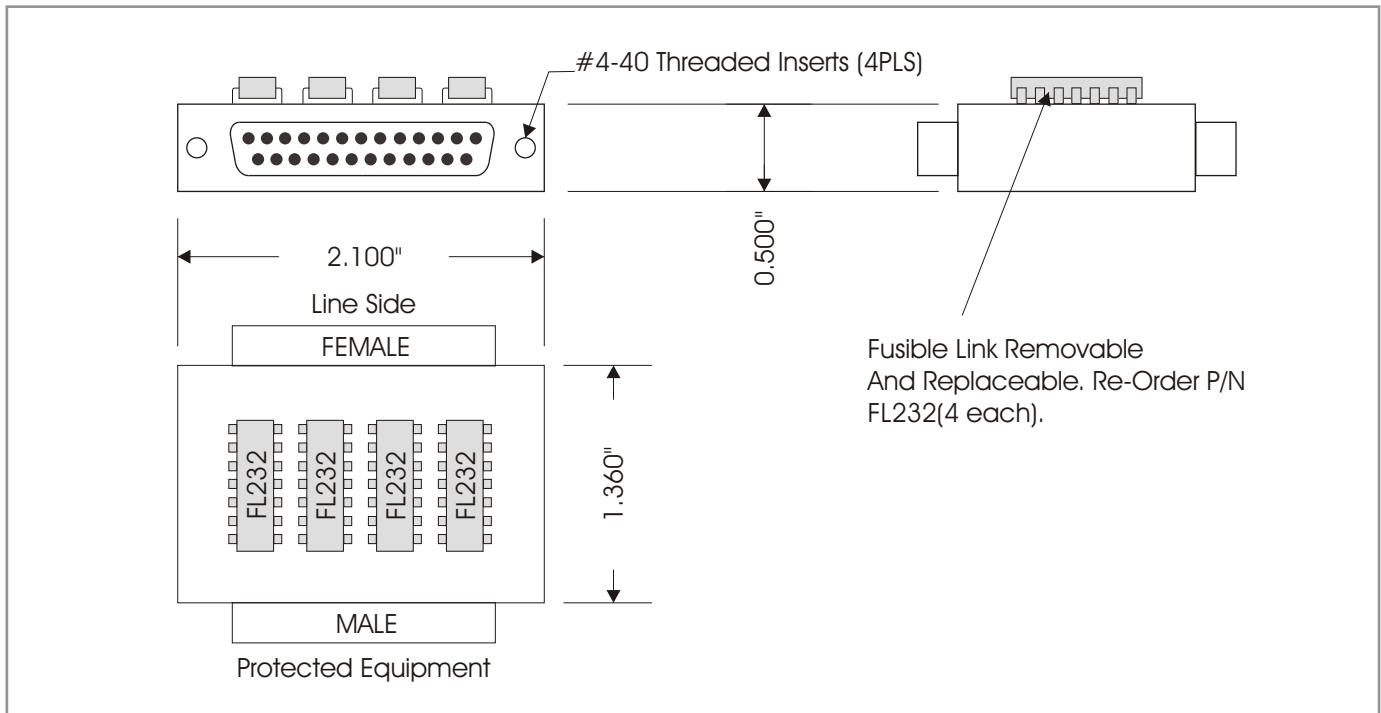
OUTLINE DRAWING
