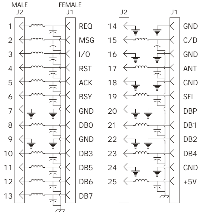
FUNCTIONAL DIAGRAM
